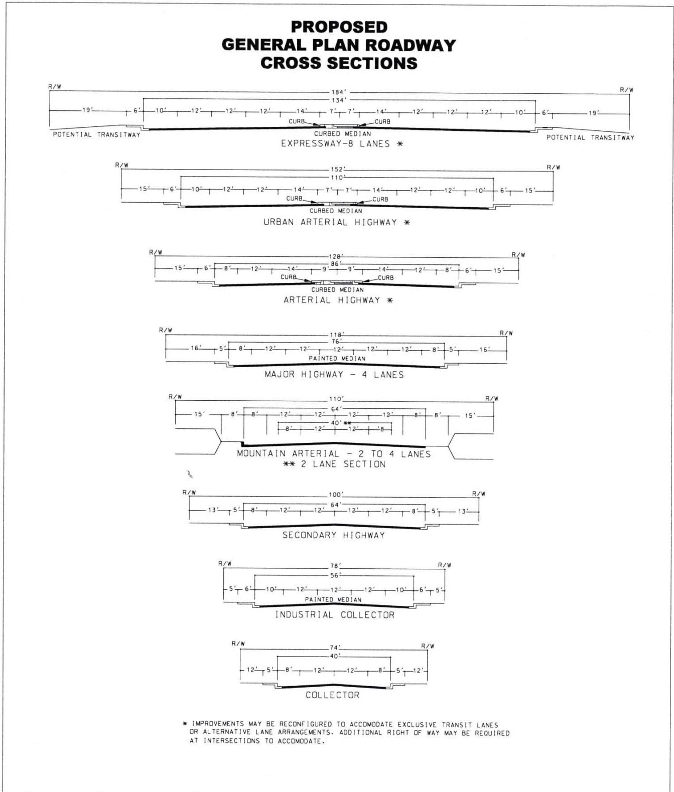
Figure C-3 Street Classification Cross-Sections
